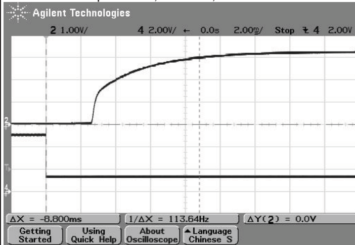
On/Off Enable Delay (Vin=48V, Vout=nom., Iout=30A, Clod=10uF, Ta=+25° C., ScopeBW=20Mhz, Trace 2=Vout, Trace 4=Enable.)
