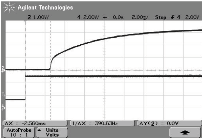
Power On Start Up (Vin=48V, Vout=nom., Iout=15A, Cload=7500uF, Ta=+25° C., ScopeBW=20Mhz, Trace 2=Vout, Trace 4=Enable)
