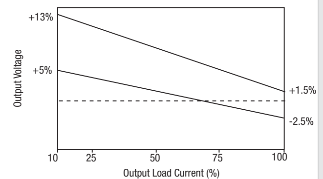
MEU1S0515ZC
