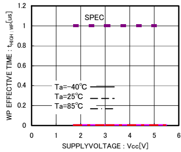
Fig.31 WP effective time t_{HIGH:WP}
