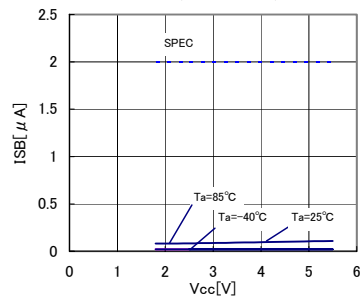
Fig.15 Standby current I_{SB}
