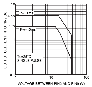
Fig.18 Safety operation range
