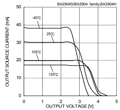
Fig.6 Output Source Current - Output Voltage (VCC=5[V])
