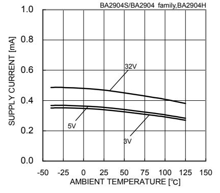
Fig.3 Supply Current - Ambient Temperature
