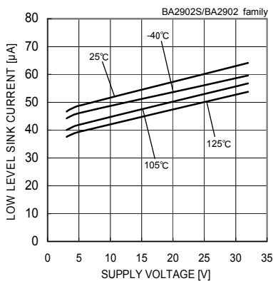
Fig. 10 Low Level Sink Current - Supply Voltage (VOUT=0.2[V])
