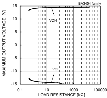
Fig.4 Maximum Output Voltage - Load Resistance (VCC/VEE=+15[V]/-15[V], Ta=25[°C])
