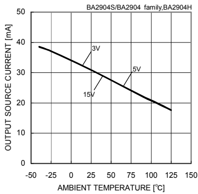
Fig.7 Output Source Current - Ambient Temperature (VOUT=0[V])
