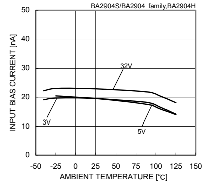
Fig. 15 Input Bias Current – Ambient Temperature (Vicm=0[V], VOUT=1.4[V])
