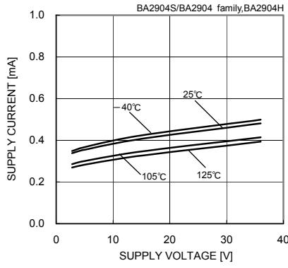
Fig.2 Supply Current - Supply Voltage
