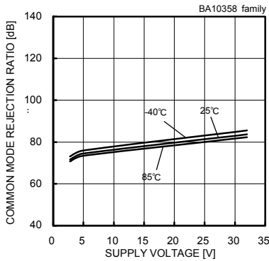
Fig. 22 Common Mode Rejection Ratio – Supply Voltage
