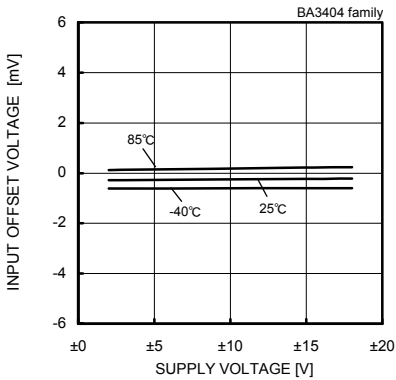
Fig.7 Input Offset Voltage - Supply Voltage (Vicm=0[V], VOUT=0[V])
