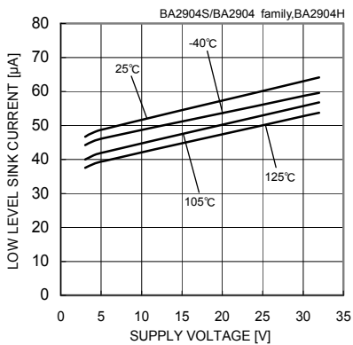
Fig.10 Low Level Sink Current - Supply Voltage (VOUT=0.2[V])
