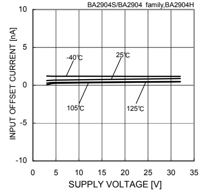
Fig. 18 Input Offset Current – Supply Voltage (Vicm=0[V], VOUT=1.4[V])
