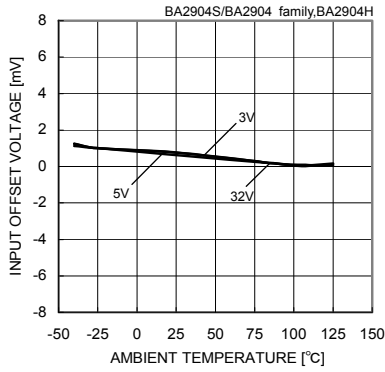
Fig. 13 Input Offset Voltage – Ambient Temperature (Vicm=0[V], VOUT=1.4[V])
