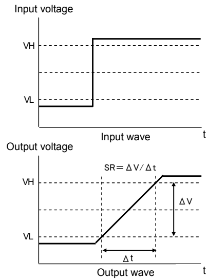
Fig.4 Slew Rate Input Waveform
