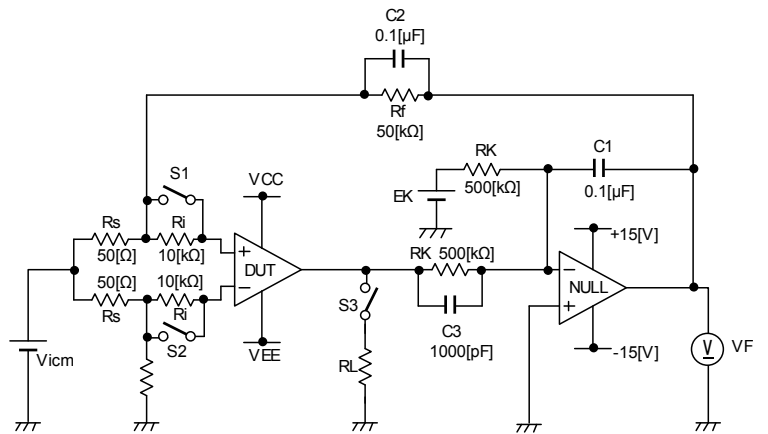
Fig.2 Measurement circuit1 (one channel only)
