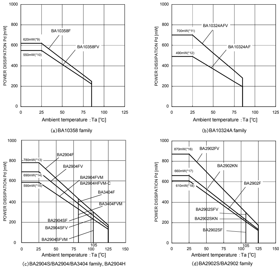
Fig.6 Thermal resistance and derating curve
