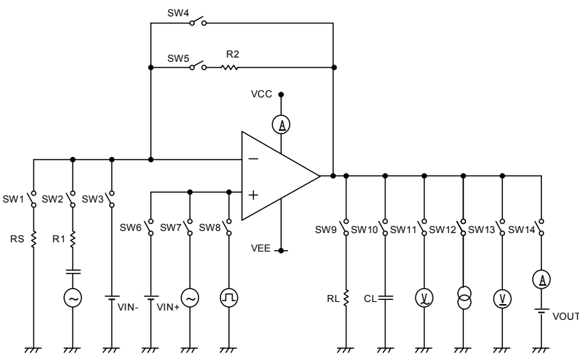
Fig.3 Measurement Circuit 2 (each Op-Amp)
