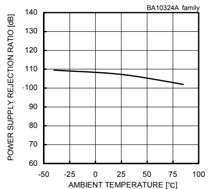
Fig. 24 Power Supply Rejection Ratio – Ambient Temperature
