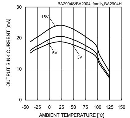
Fig.9 Output Sink Current - Ambient Temperature (VOUT=VCC)
