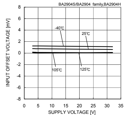
Fig.12 Input Offset Voltage - Supply Voltage (VICM=0[V], VOUT=1.4[V])
