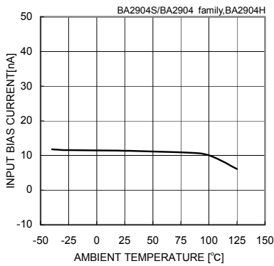
Fig. 16 Input Bias Current – Ambient Temperature (VCC=30[V], Vicm=28[V], VOUT=1.4[V])
