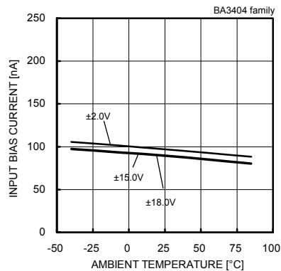
Fig.10 Input Bias Current - Ambient Temperature (Vicm=0[V], VOUT=0[V])
