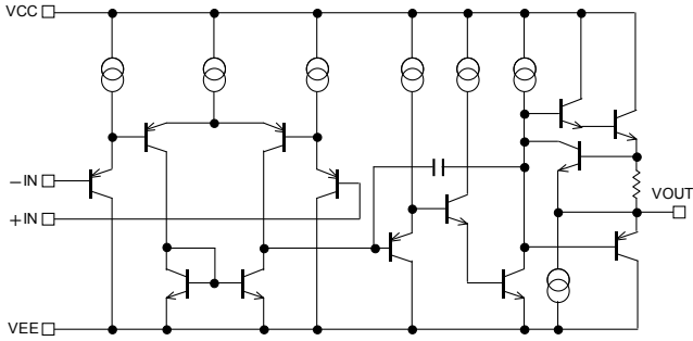
BA10358/BA10324A/BA2904S/BA2904/ BA2902S/BA2902/BA2904H simplified schematic
