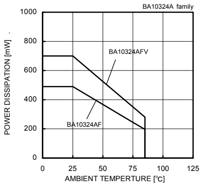
Fig.1 Derating Curve
