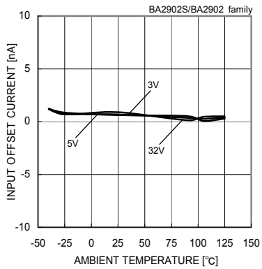
Fig. 19 Input Offset Current – Ambient Temperature ( V_{icm}=0[V] , V_{OUT}=1.4[V] )
