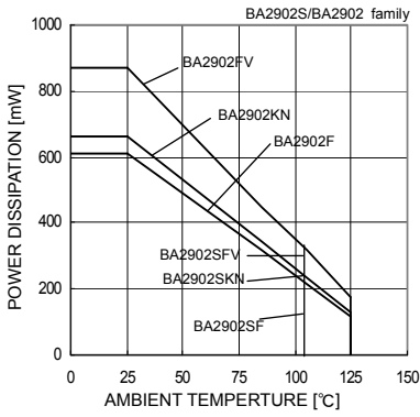
Fig. 1 Derating Curve
