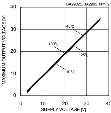
Fig. 4 Maximum Output Voltage - Supply Voltage (RL=10[kΩ])
