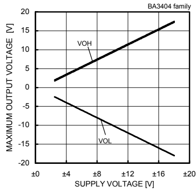
Fig.5 Maximum Output Voltage - Supply Voltage
