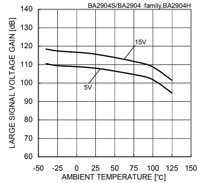
Fig. 21 Large Signal Voltage Gain – Ambient Temperature (RL=2[kΩ])
