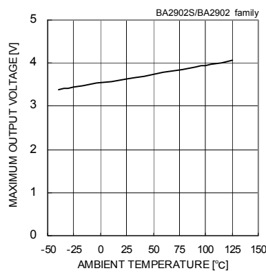
Fig. 5 Maximum Output Voltage - Ambient Temperature (VCC=5[V], RL=2[kΩ])
