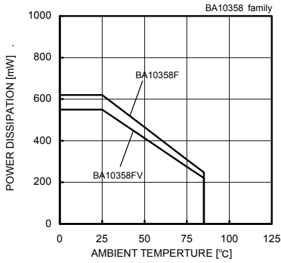
Fig.1 Derating Curve
