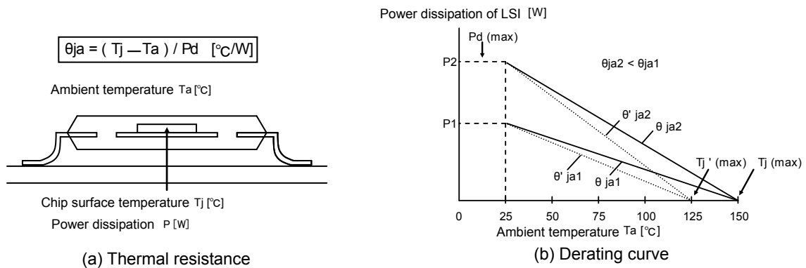
Fig.6 Thermal resistance and derating curve
