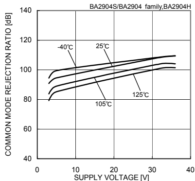
Fig. 22 Common Mode Rejection Ratio – Supply Voltage
