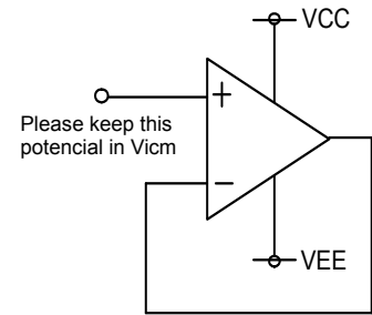
Fig.1 Example of processing unused circuit
