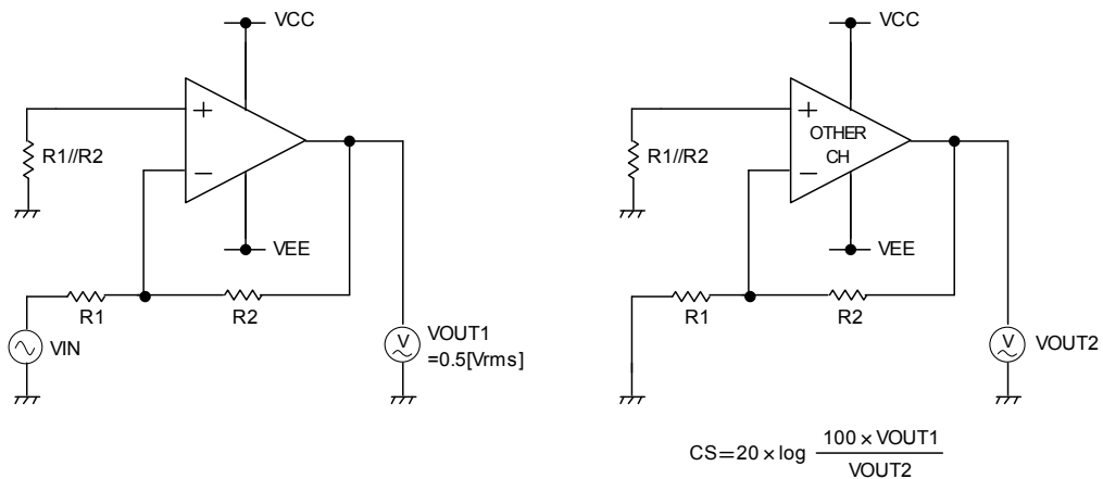
Fig.5 Measurement Circuit 3
