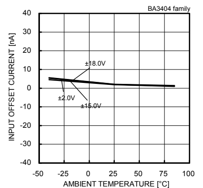
Fig.12 Input Offset Current - Ambient Temperature (Vicm=0[V], VOUT=0[V])
