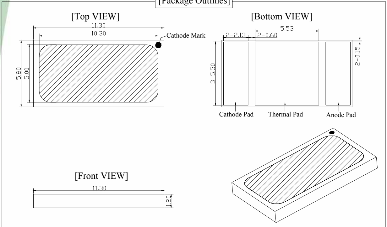
[Package Outlines]
