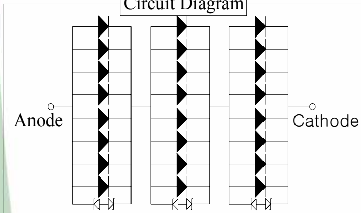
[Circuit Diagram]
