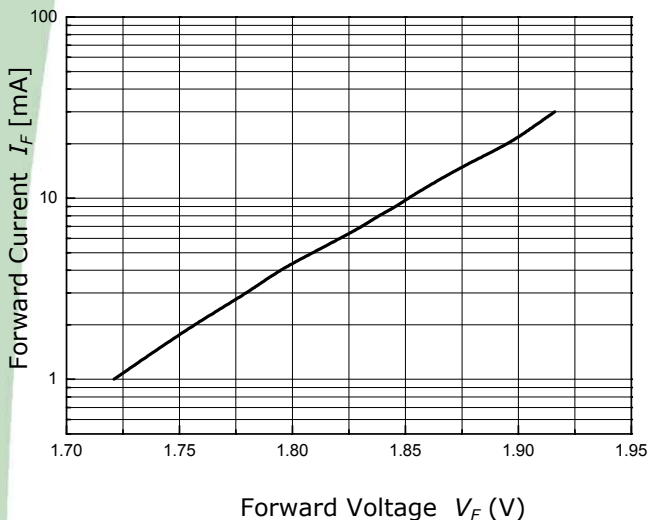
Forward Current vs. Forward Voltage ( T_a=25\text{ }^\circ\text{C} )
