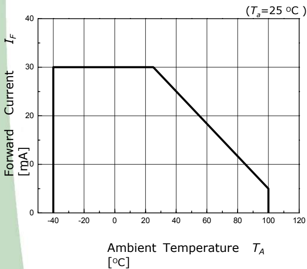
Forward Current Derating Curve ( T_a=25\text{ }^\circ\text{C} )
