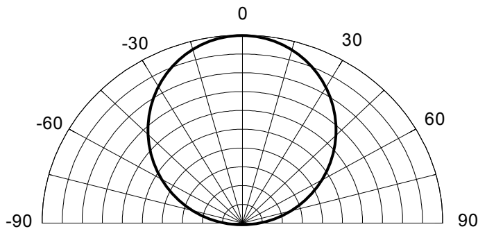
Radiation Diagram
