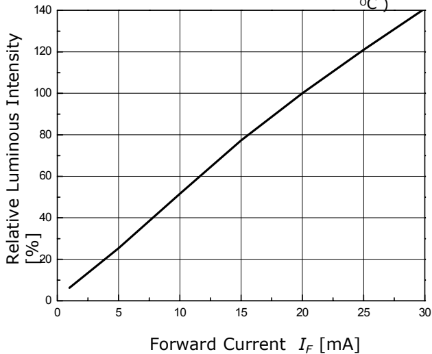
Relative Luminous Intensity vs Forward Current ( T_a=25\text{ }^\circ\text{C} )
