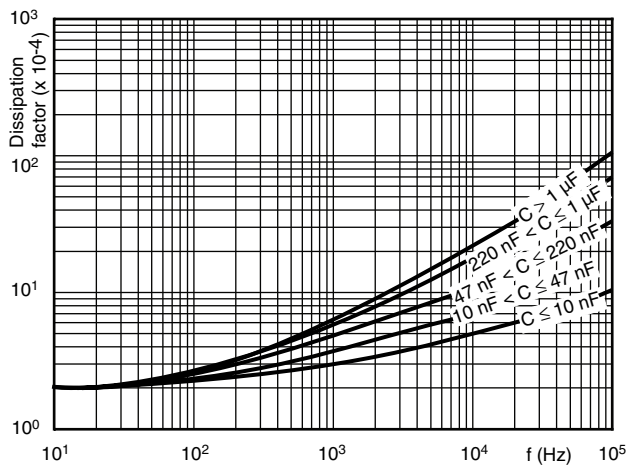
Tangent of loss angle
