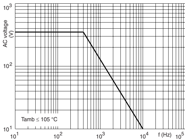
Max. RMS voltage and current as a function of frequency
