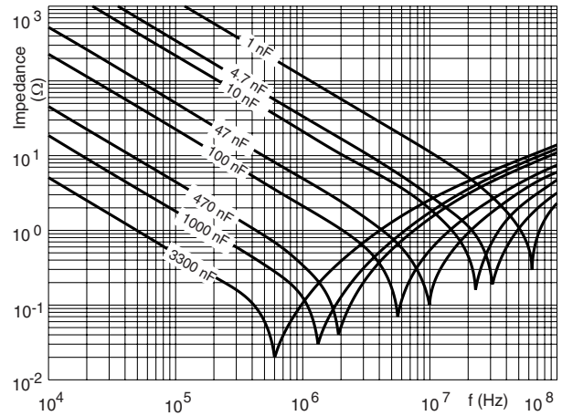
Impedance
