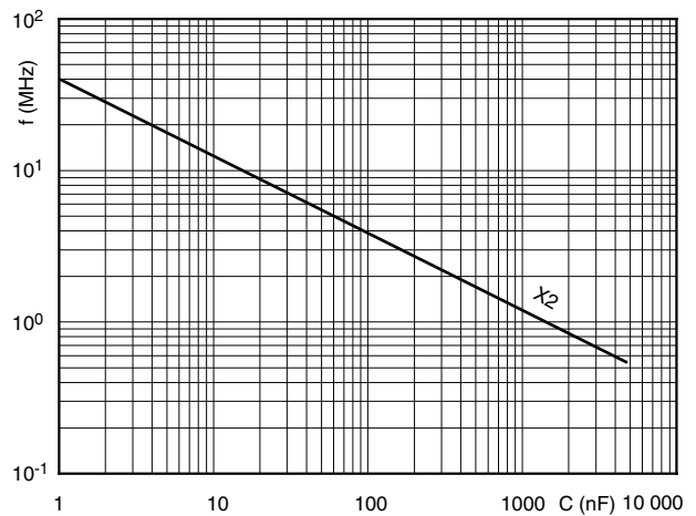
Resonant frequency
