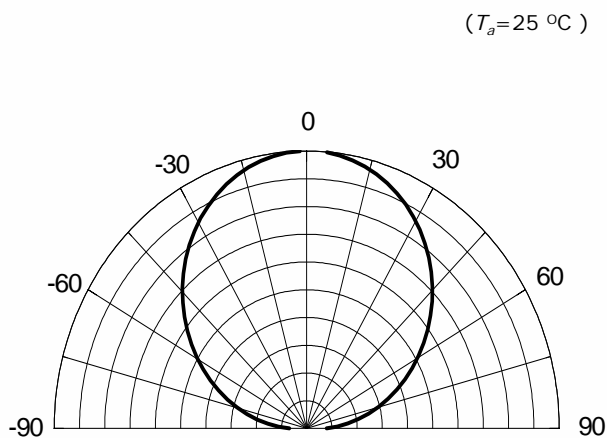
Radiation Diagram
