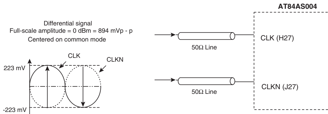
Figure 11-7. AT84AS004 Clock Input Recommended Termination Scheme (Differential)
