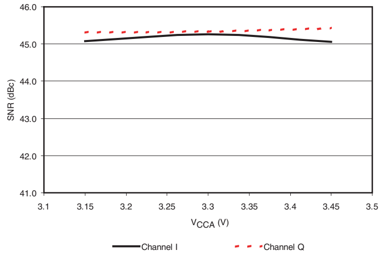
Figure 9-20. SNR Versus V_{CCA} ( F_s = 500 Mps, F_{in} = 250 MHz, 1:2 DMUX, F_s/4 DR Type, ISA = 0 ps)
