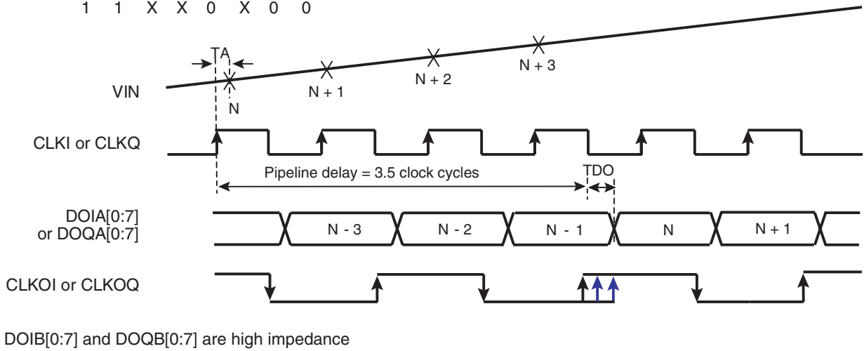
Figure 7-4. 1:2 DMUX Mode, Clock I = ADC I, Clock I = ADC Q
