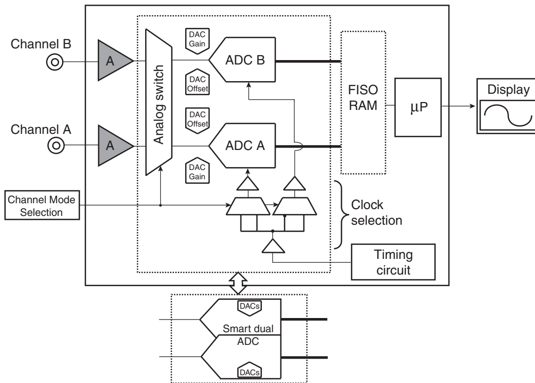
Figure 6-2. Dual Channel Digital Oscilloscope Application
