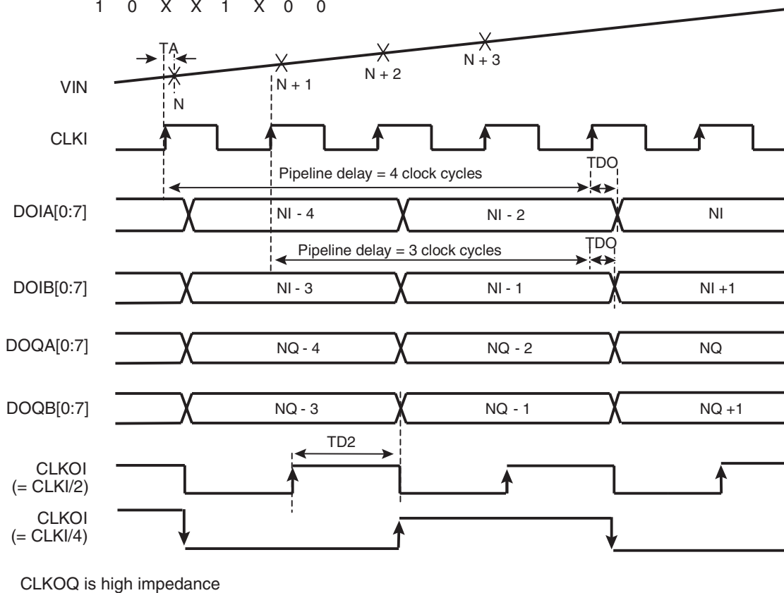
Figure 7-4. 1:2 DMUX Mode, Clock I = ADC I, Clock I = ADC Q
