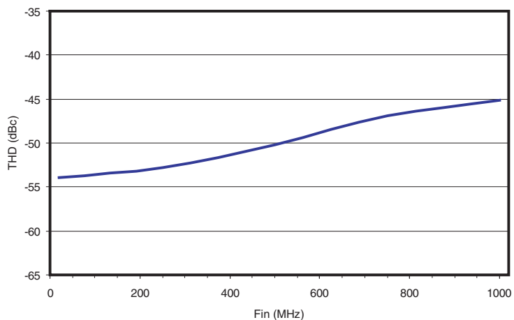
Figure 9-15. THD Versus Input Frequency ( F_s = 1 Gps)
