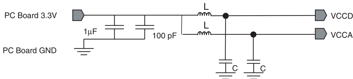
Figure 13-1. V_{CCD} and V_{CCA} Bypassing and Grounding Scheme
