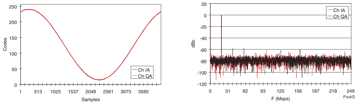
Figure 9-17. F_s = 1 Gps and F_{in} = 20 MHz (1:2 DMUX, F_s/2 DR Type, F_{iSDA} = -15 ps, I_{SA} = -50 ps)
