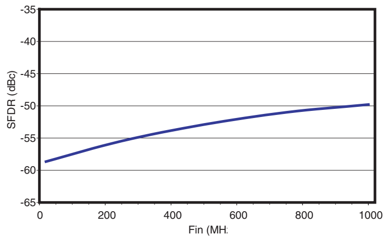
Figure 9-14. SFDR Versus Input Frequency ( F_s = 1 Gsps)
