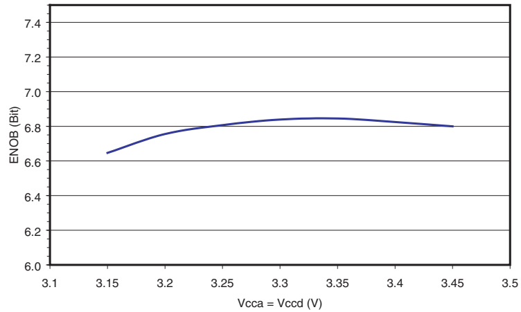
Figure 9-22. ENOB Versus V_{CCA} = V_{CCD} ( F_s = 1 Gsps, F_{in} = 500 MHz, 1:2 DMUX, F_s/4 DR Type, ISA = -50 ps)
