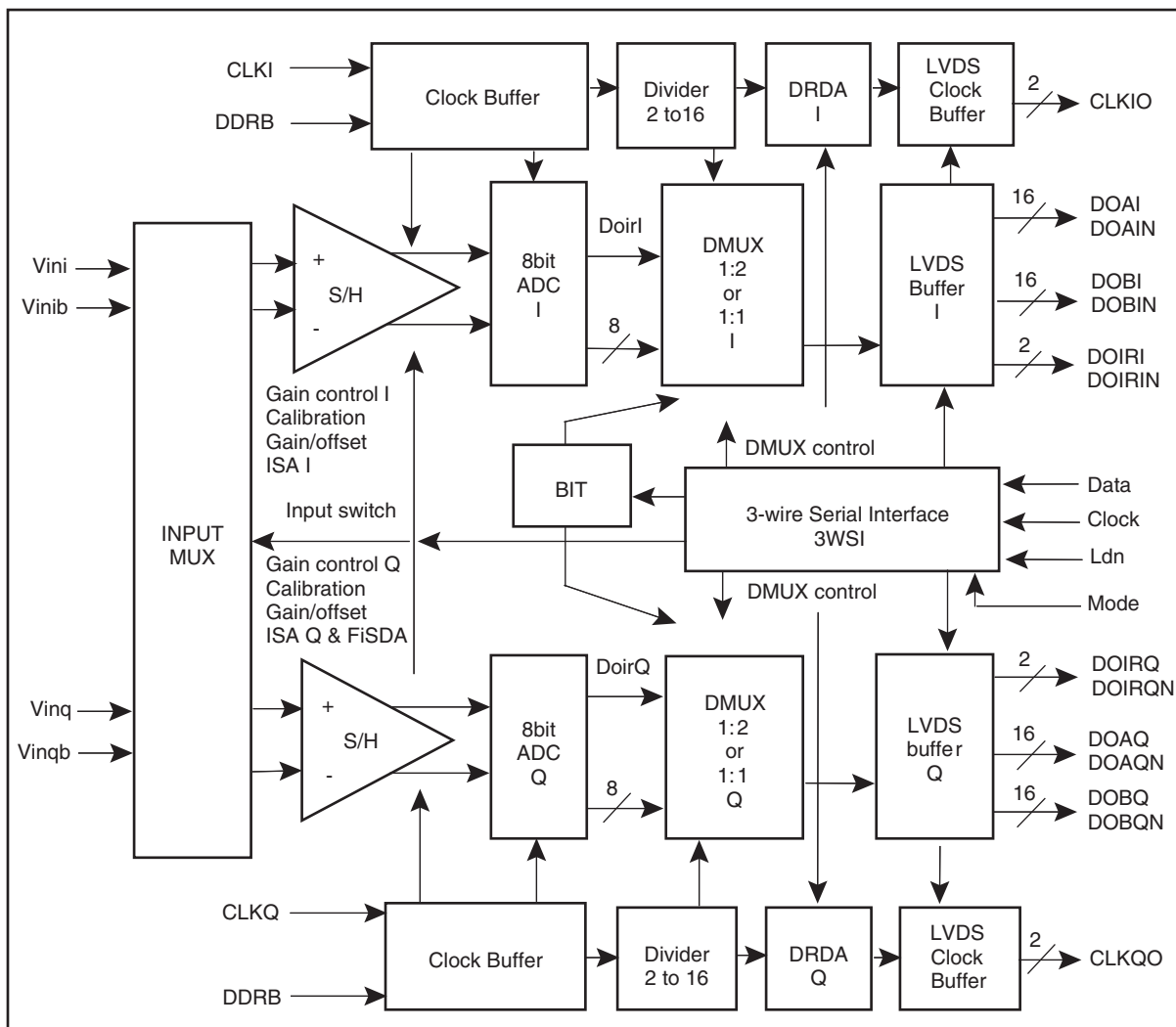
Figure 5-1. Simplified Block Diagram
