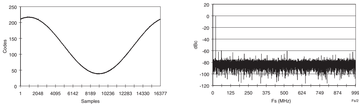
Figure 9-20. F_s = 1 Gps and F_{in} = 20 MHz (Interleaving Mode F_{int} = 2 Gps, F_s/4 DR Type, F_iSDA = -15 ps, ISA = -50 ps)
